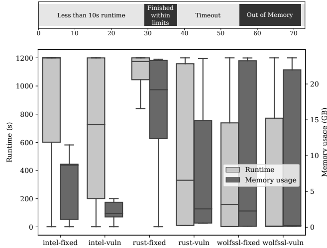
Figure 4.15: Runtime and memory usage of the benchmarked enclaves.
