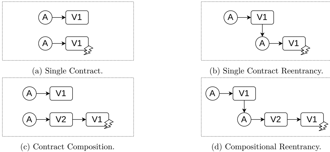
Figure 5.5: Different settings illustrating the difference and similarities between reentrancy and compositional attacks.
